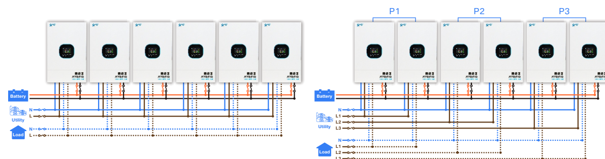
Parallel Operation in Single phase
